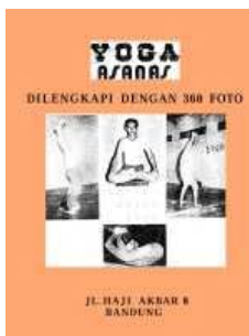
Yoga Asanas
